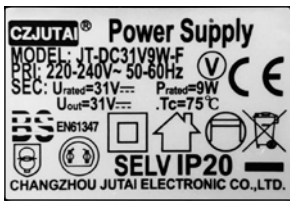
Transformer data plate
